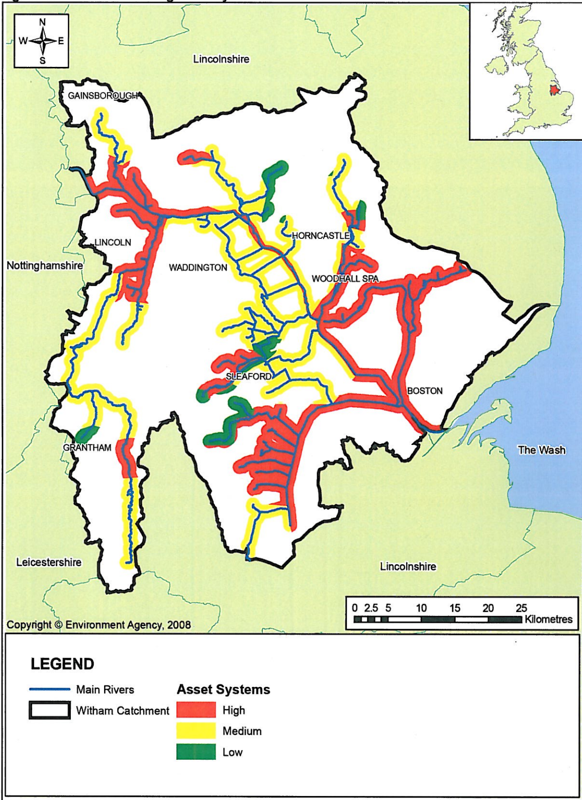
Figure 3.9: Flood risk management systems in River Witham CFMP area
